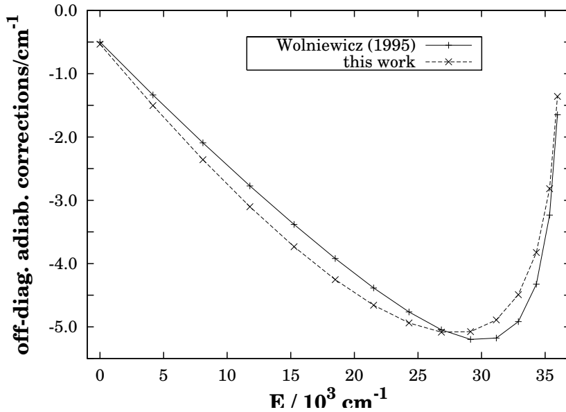
Figure 1. Non-adiabatic corrections in \text{H}_2
